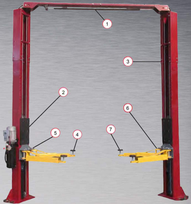
DM9CF Symmetric/Asymmetric Clear Floor Two Post Lift
