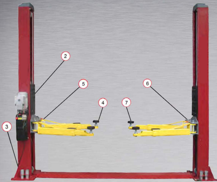
DM9BP Symmetric Floor Plate Two Post Lift
